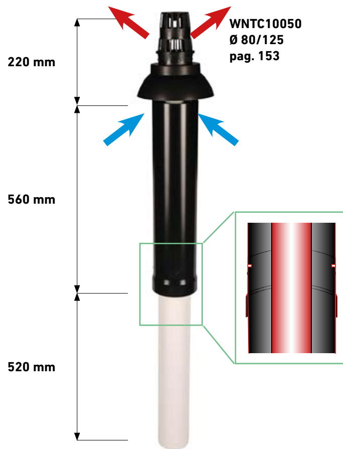
Installation on flat roofs with N5-TN13 tile
